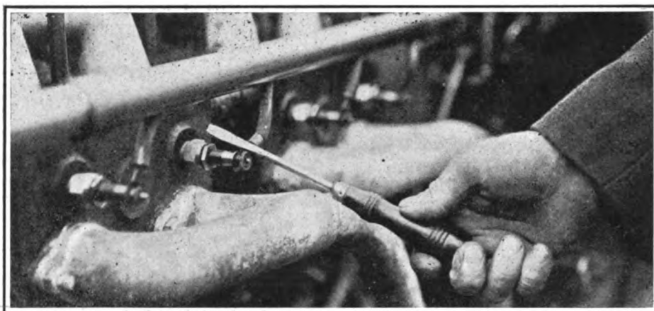
FIG 8.—INCORRECT WAY, TOOL TOUCHING PLUG TERMINAL FIRST.
